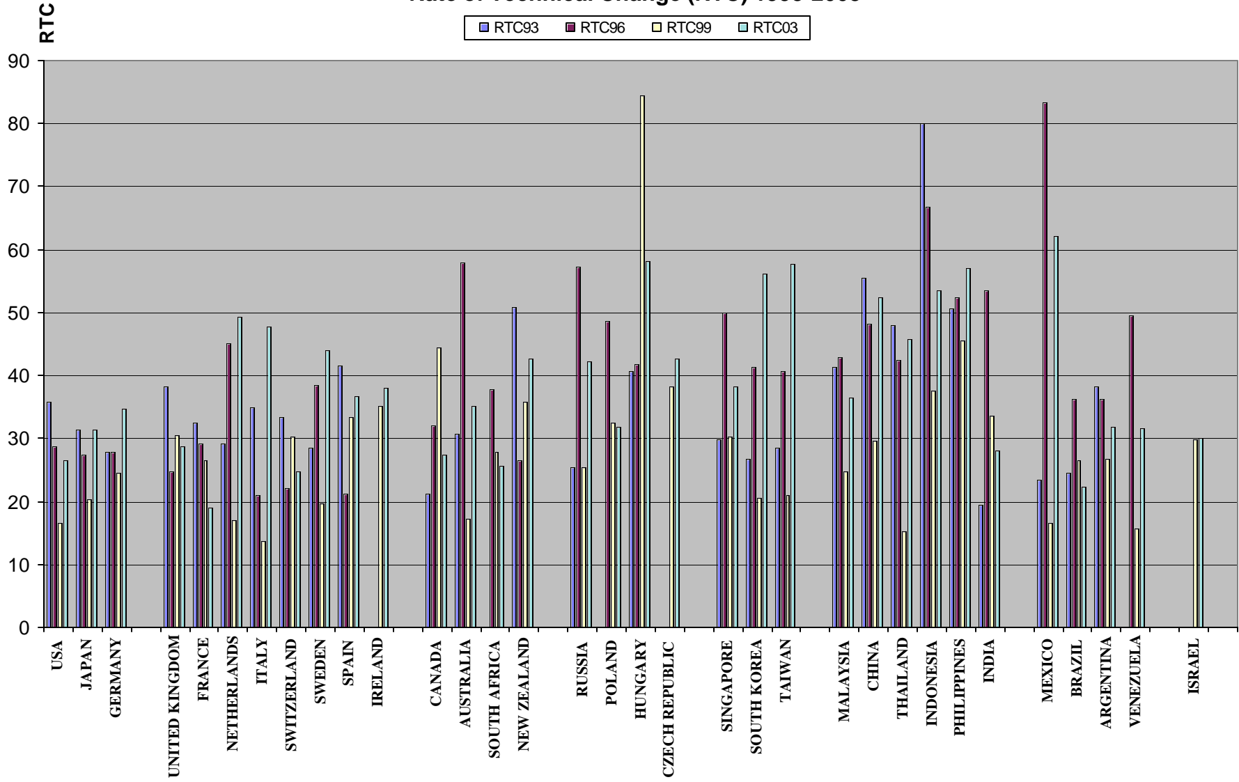
Figure 17 Rate of Technical Change (RTC) 1993-2003
