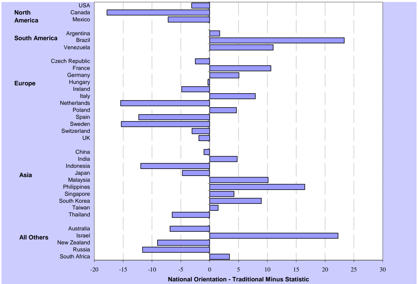
Figure 20: Difference Scores, Traditional Minus Statistics-only for National Orientation 2005 (NO-05)
